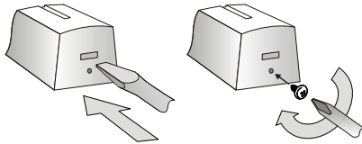
Fig. 2 Opening the detector cover and securing it with a screw
